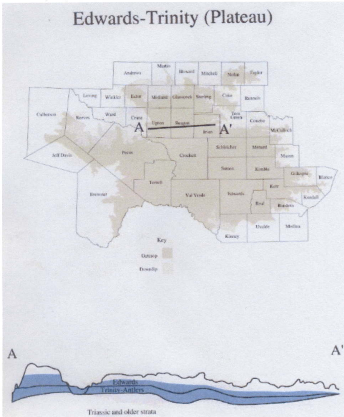
Figure 3: Aerial extent of the Edwards-Trinity (Plateau) Aquifer in Texas (Adapted from Ashworth and Hopkins, 1995)
